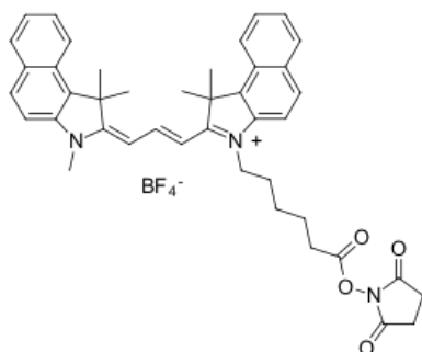
Structure of Cyanine3.5 NHS ester
